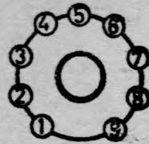
Noval B9A
